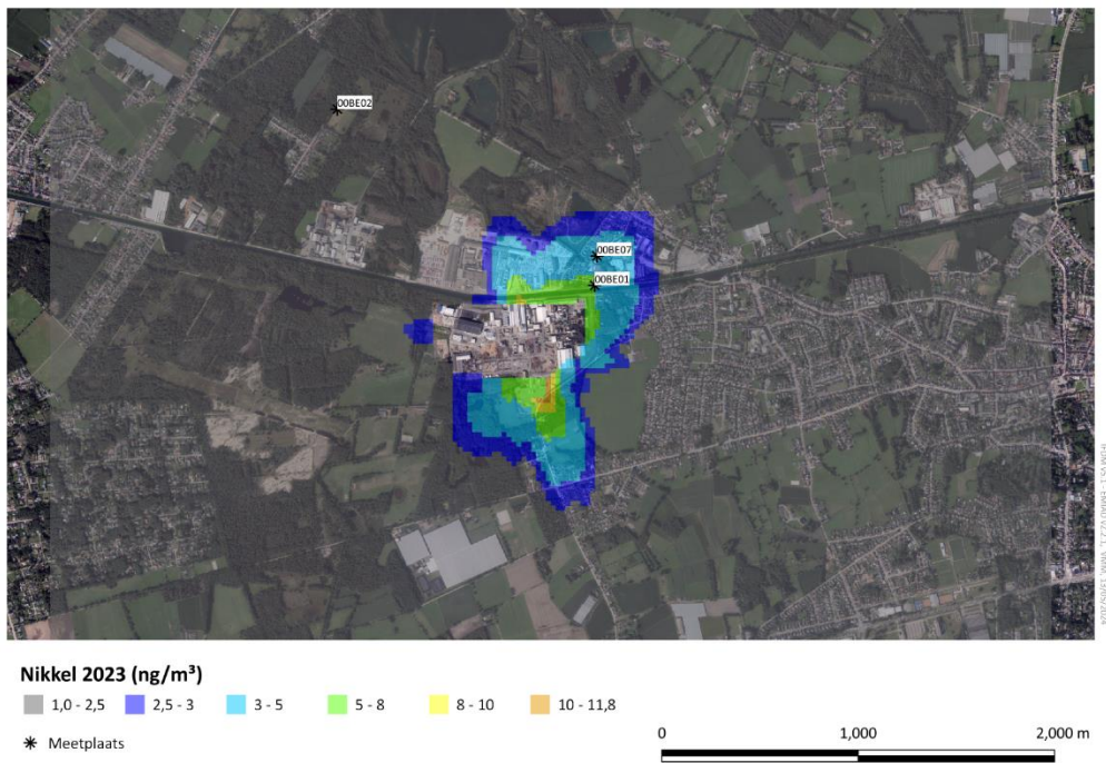
Figuur 6: Modellerings nikkels in 2023
